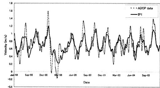
(b) W-E velocity component in IP2 model
