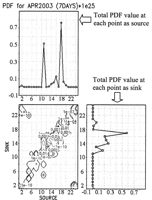
Fig.4 Matrix connectivity expressed in probability density function (PDF) (lower left panel) after 7 days released from April 1st, 2003. Upper and lower right panels show the total PDF values as source and sink, respectively, for each point.
