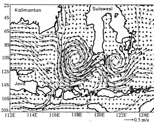
Fig.2 Surface current vectors showing pattern of eddies around Lombok-Flores Sea regions in February 2006 (during positive Indian Dipole mode).
