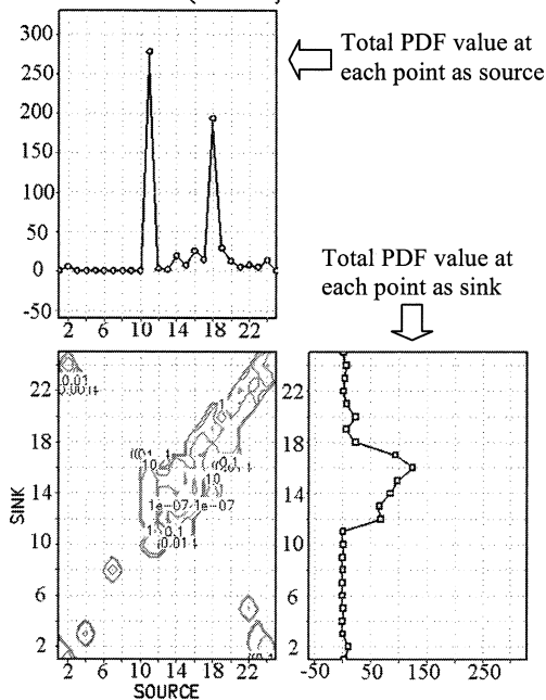
Fig.5 Similar to Fig. 4, but after 14 days released.
