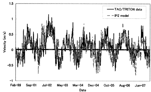
Fig 1. Examples of validation results for W-E velocity component for (a) IP1 model ( 0^0, 110^0W ) and (b) IP2 model ( 2^0N, 147^0W ).
