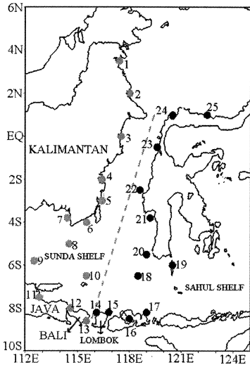
Fig.3 Larval clouds with the initial concentration of 0.05 \text{ mmol N m}^{-3} were released at the 25 places around the central part of Indonesian seas. Points 1-13 are located in Sunda continental shelf, while points 14-25 are located in Sahul continental shelf. Dashed line represents the virtual "Wallace line"
