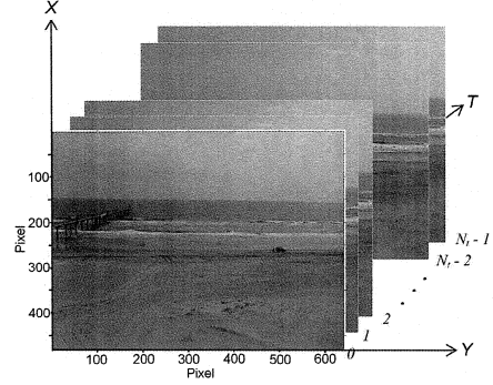
Fig. 2 Snapshot image around pier area
