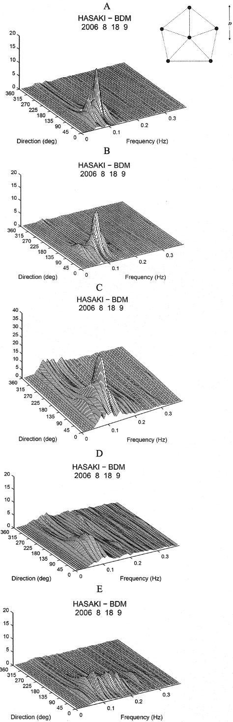
Fig. 6 Variation the directional wave spectrum along a cross shore transect on Hasaki beach (insert: polygon array)
