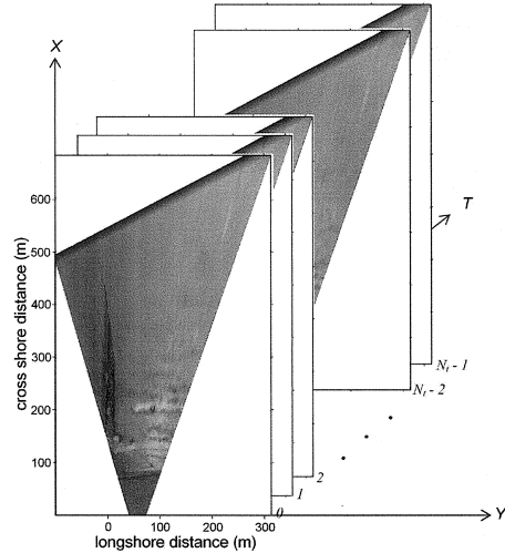
Fig. 4 Rectified image time series from snapshot images on 18 August 2006 at 09.00 h around pier area.
