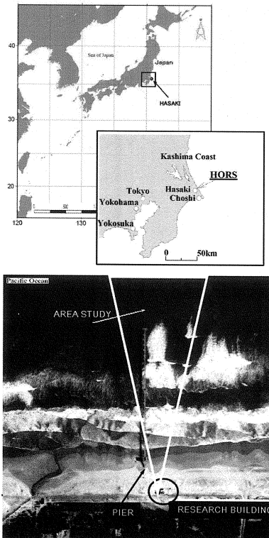
Fig. 1 Location of the Hasaki site (top) and aerial photo of the field site (bottom) with the view angle of study area indicated by triangle area
