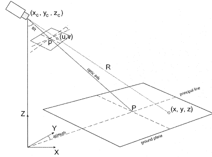
Fig. 3 Relation between image coordinate (u, v) and real world coordinate (x, y, z)
